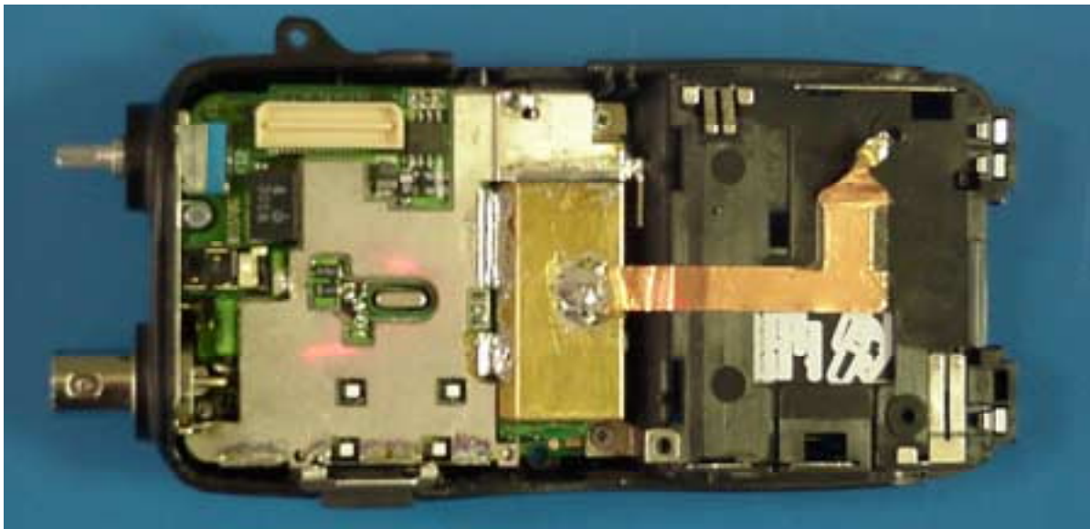
FRONT VIEW RF PCB BOARD
