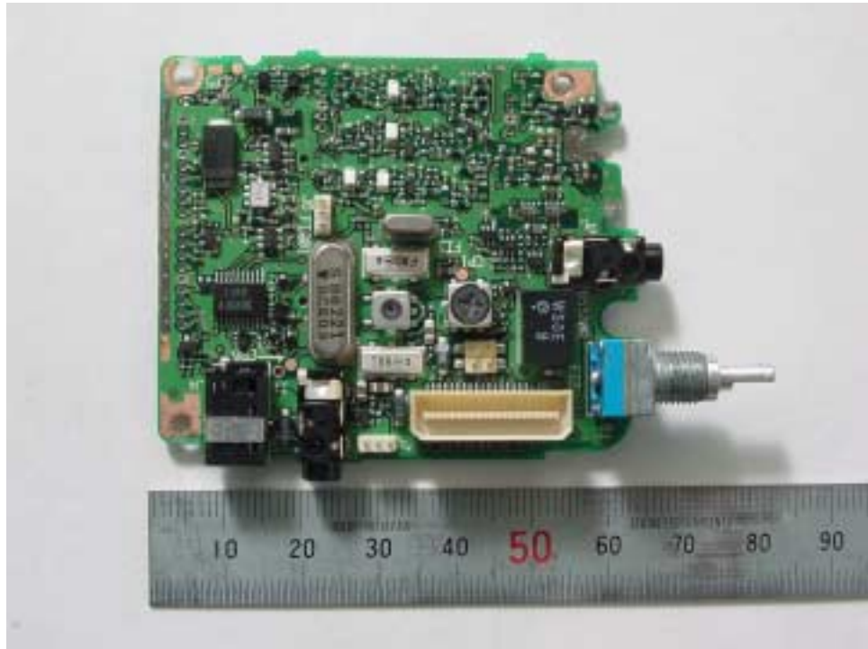
FRONT VIEW RF PCB
