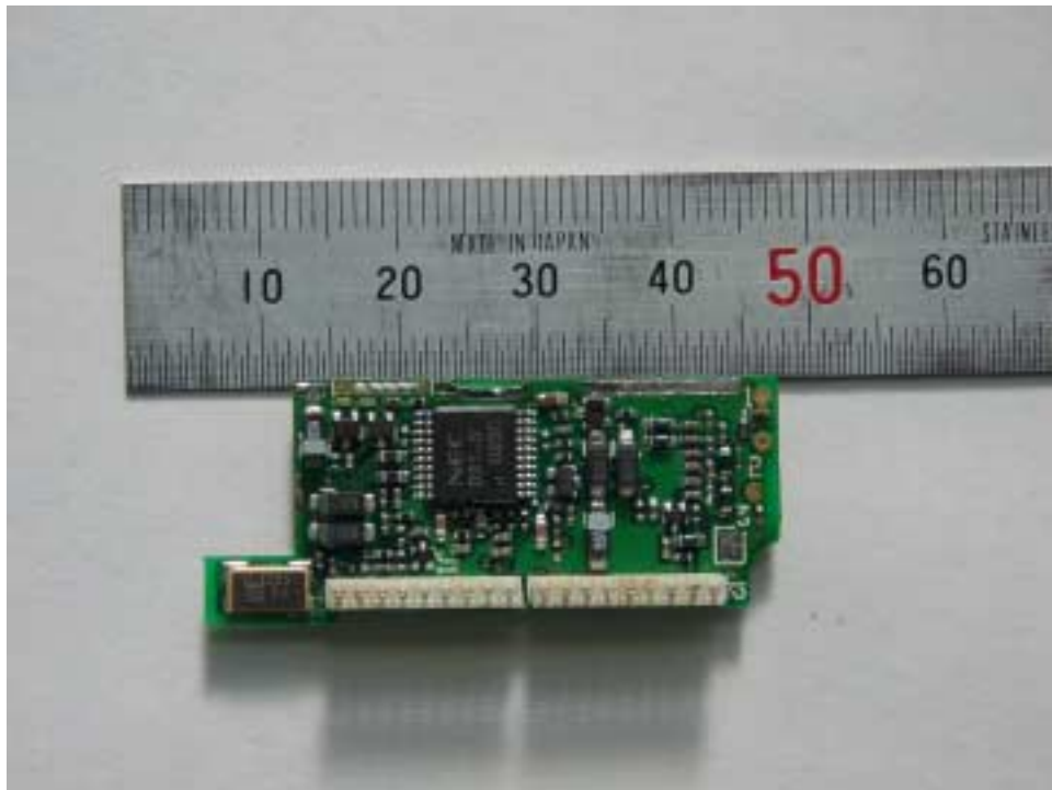
FRONT VIEW VCO
