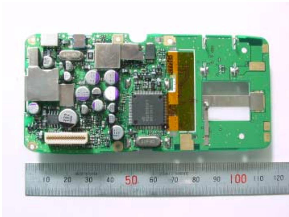
REAR VIEW LOGI PCB
