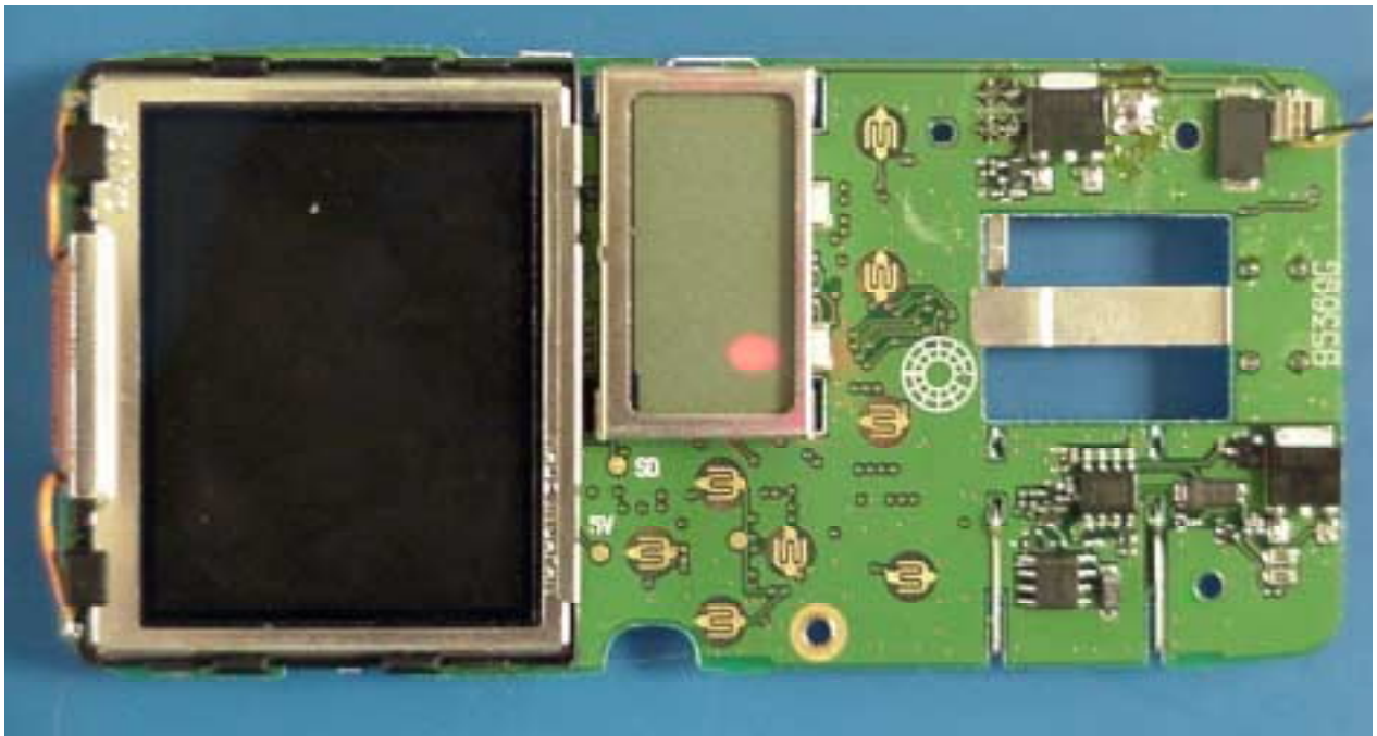
FRONT VIEW MAIN PCB BOARD WITH LCD
