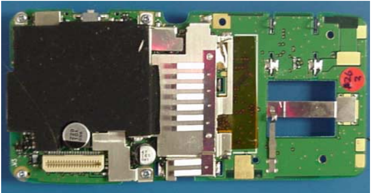
REAR VIEW MAIN PCB BOARD WITH LCD
