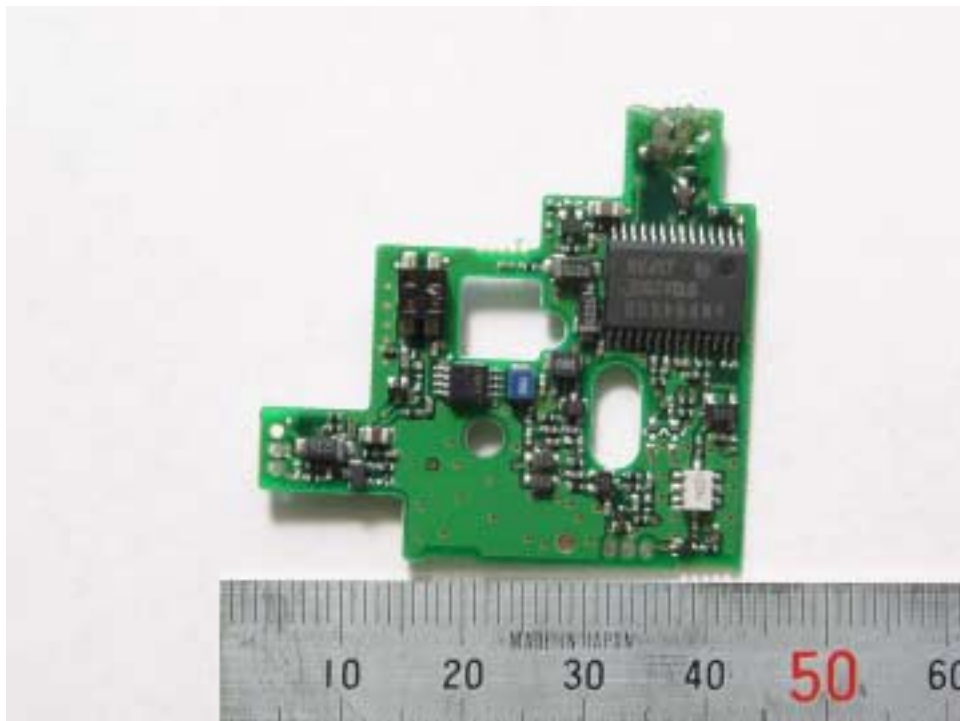
REAR VIEW FM TV PCB
