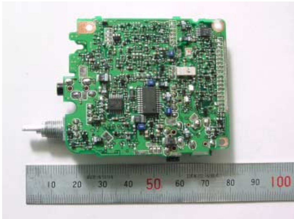
REAR VIEW RF PCB
