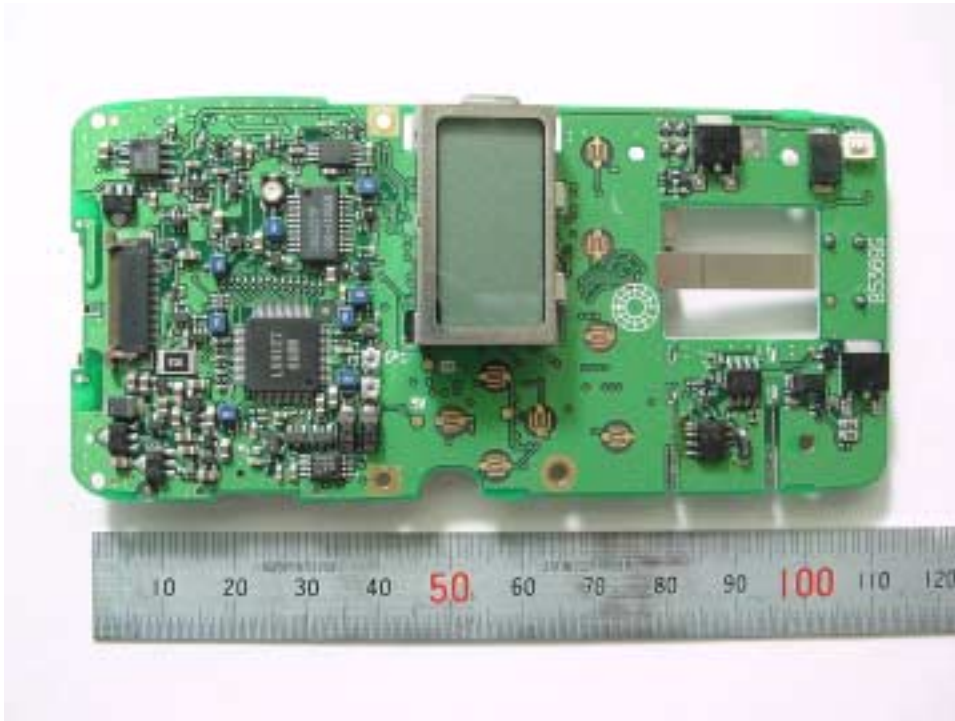
FRONT VIEW LOGI PCB
