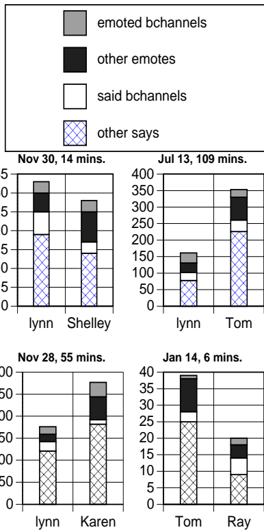
Figure 1: Ratios of Says to Back Channels and Other Emotes in Two-Party Conversations
